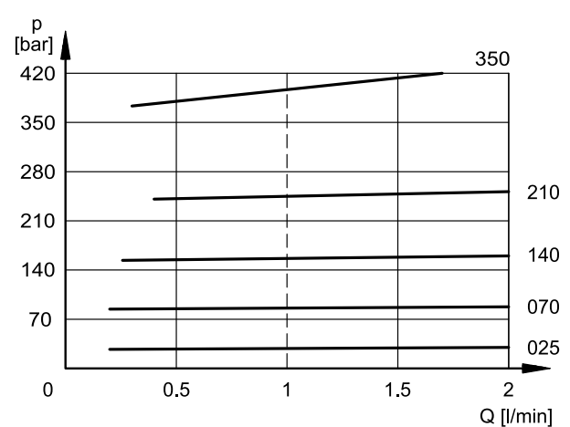
PRESSURE VARIATION p_{\text{max}} = f(Q)
