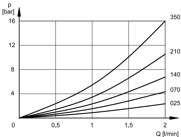
MINIMUM CONTROLLED PRESSURE p_{\text{min}} = f(Q)
