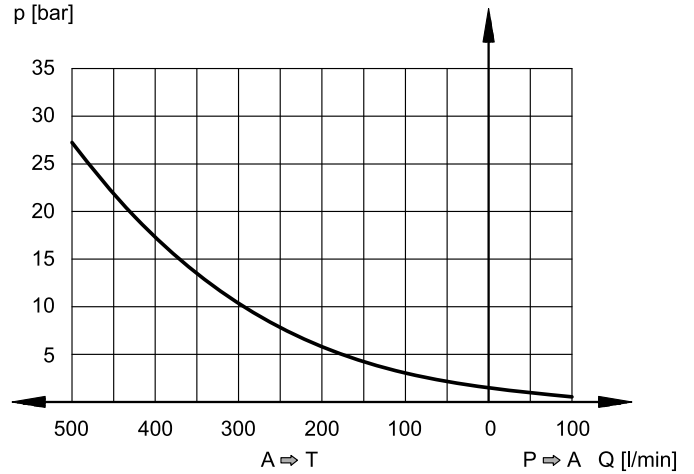
MIN. CONTROLLED PRESSURE p_{min} = f(Q)
