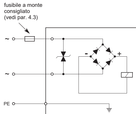
Bobina RAC
