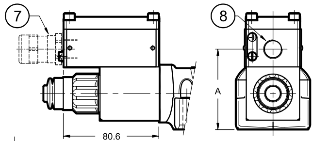
DL5BK*-*/10*-*K9S*/CM
