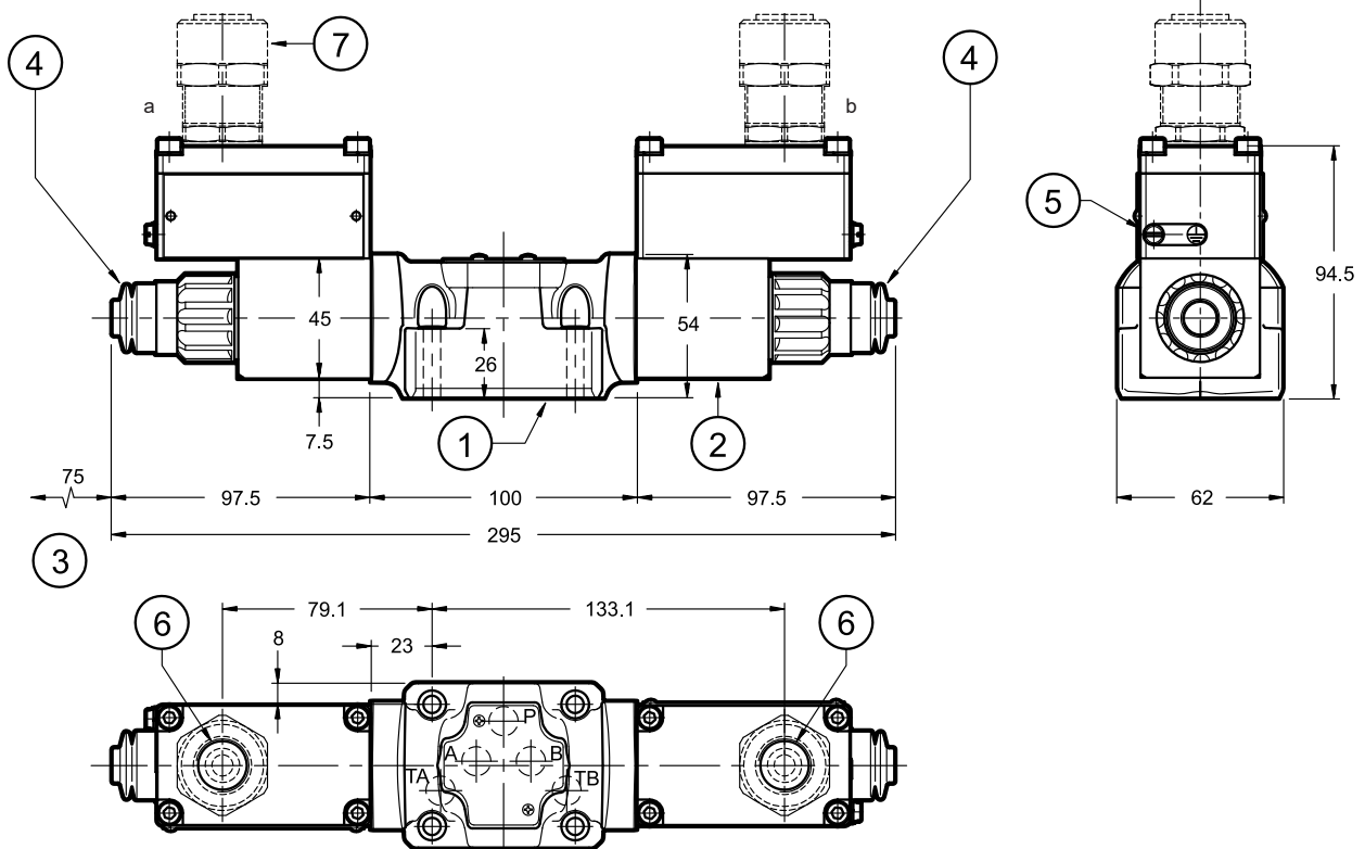
DL5BK*-*/10*-*K9S*/CM
