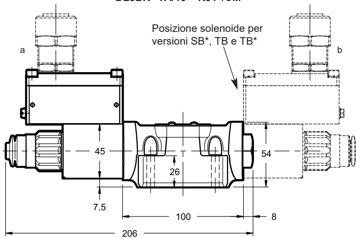
DL5BK*-SA*/10*-*K9T*/CM DL5BK*-TA/10*-*K9T*/CM
